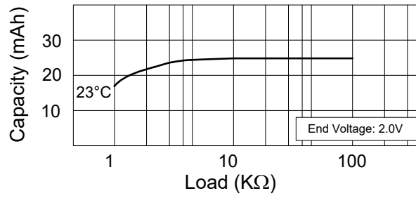
Figure 2. Load-Capacity
