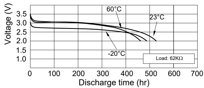
Figure 4. Temperature Characteristics
