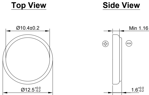
Figure 7. SCR1216 Mechanical Layout
