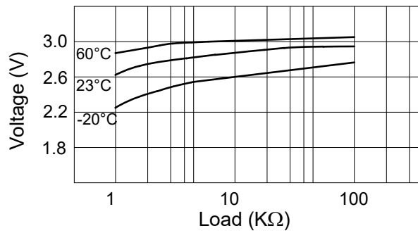
Figure 5. Load-Operating voltage
