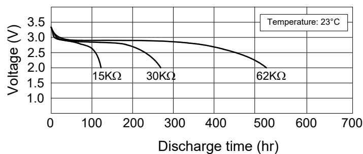
Figure 1. Discharge Characteristics
