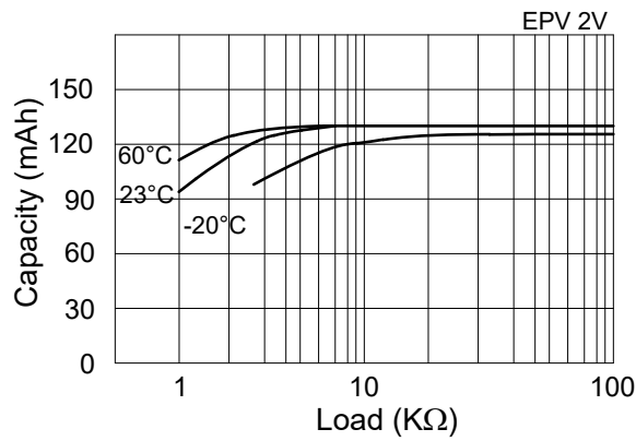
Figure 5. Load-Capacity
