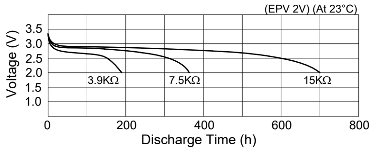
Figure 1. Discharge Characteristics
