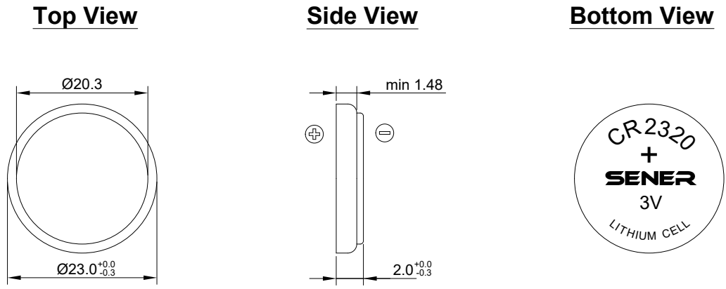
Figure 7. SCR2320 Mechanical Layout
