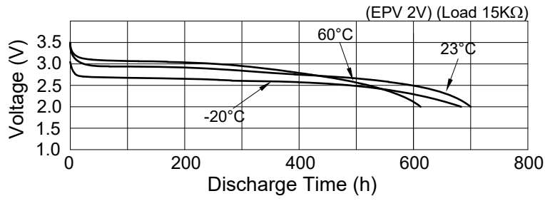
Figure 4. Temperature Characteristics
