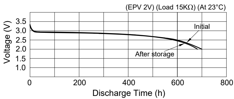
Figure 6. Storage Characteristics
