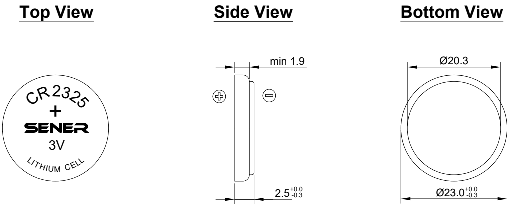
Figure 7. SCR2325 Mechanical Layout
