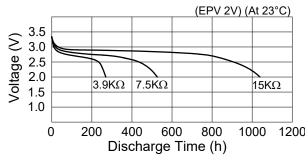
Figure 1. Discharge Characteristics
