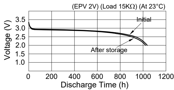
Figure 6. Storage Characteristics
