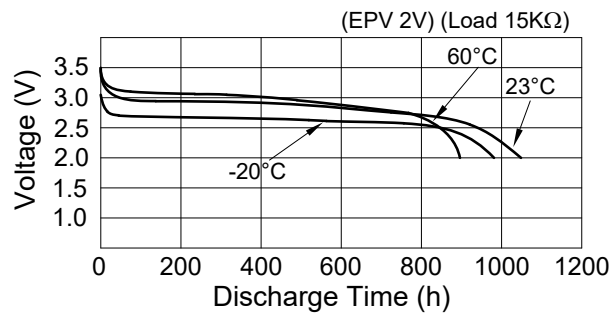
Figure 4. Temperature Characteristics
